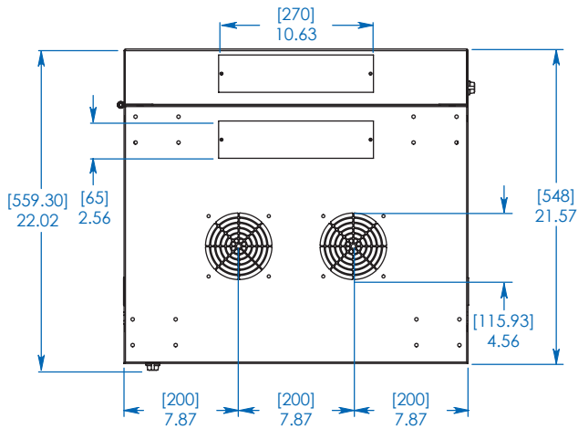
TOP/BOTTOM VIEW
